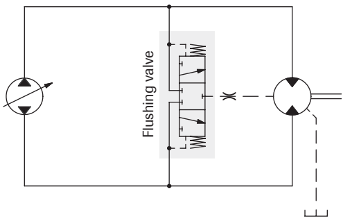
Simplified circuits
